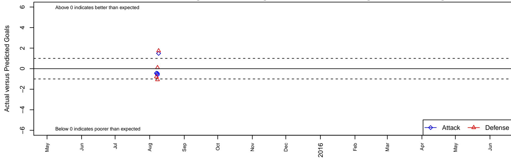
Junior Rangers Academy B03 Dots are actual minus expected GF (blue circles) and GA (red triangles). Blue line is smoothed change in attack strength. Red is smoothed change in defense strength.
